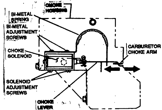
Figure 5-3 — Generac Automatic Choke
