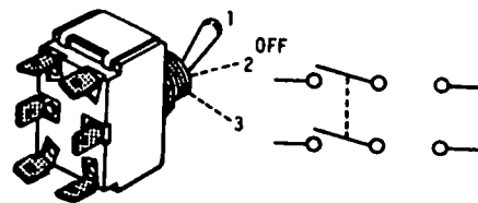
Figure 3-5 — Double Pole, Double Throw Switch
