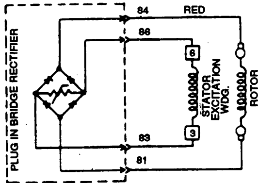
Figure 2-5 — Direct Excited Units
