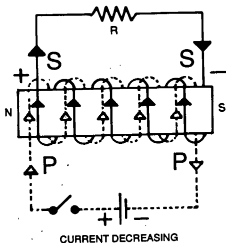
Figure 7-1 — The Principle of Mutual Induction
