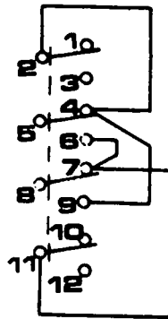
Figure 3-7 — Four-Pole, Double Throw Switch
