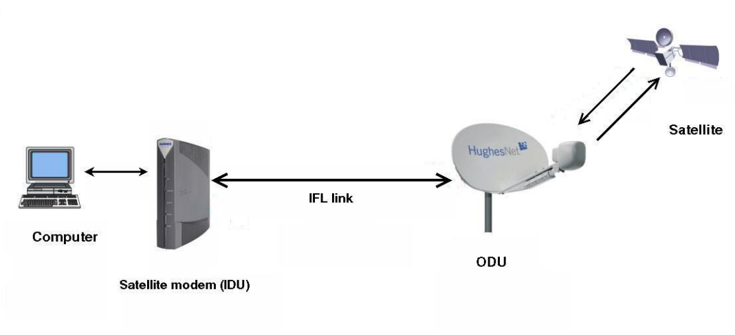
Figure 3: Satellite modem and related components
