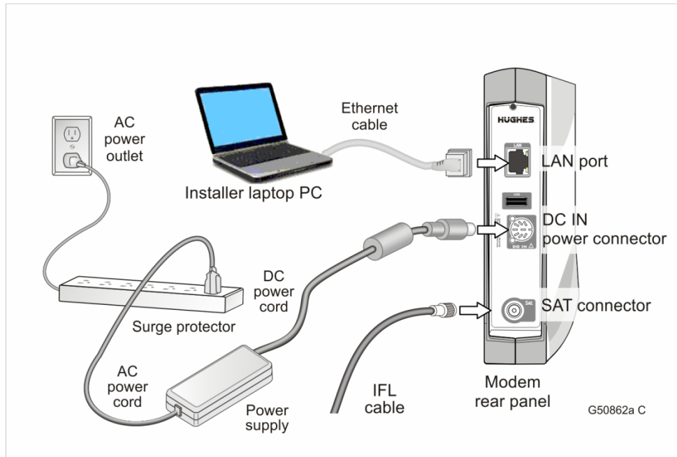
Figure 18: All connections completed
