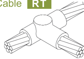
Tee of Horizontal Run & Tap Cables
