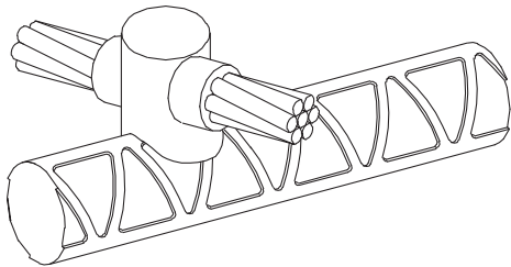
Cross of Horizontal Cable Lapped Over Horizontal Rebar
