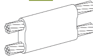
Parallel Thru Splice of Horizontal Cables, Tap Conductor Over Run
