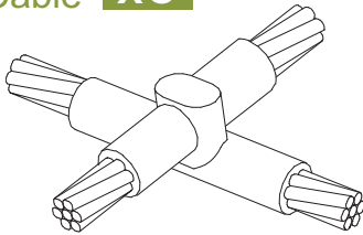
Cross of Horizontal Cables, Lapped and Not Cut
