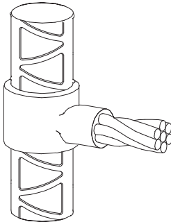
Tee of Vertical Thru Rebar & Horizontal Tap Cable
