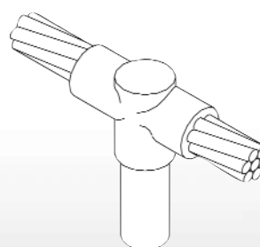
Horizontal Thru Cable to Top of Ground Rod
