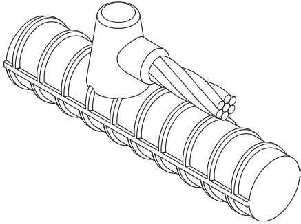
Parallel Cable Tap of Horizontal Cable to Thru Horizontal Rebar
