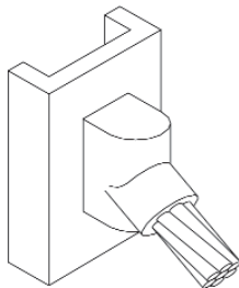
Cable Down at 45° to Vertical Flat Steel Surface
